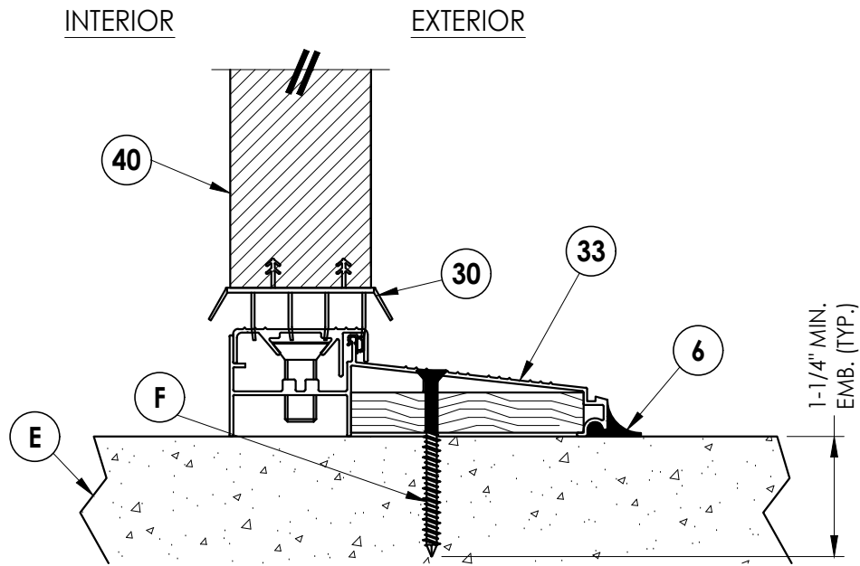
3 VERTICAL CROSS SECTION 5 Inswing configuration
