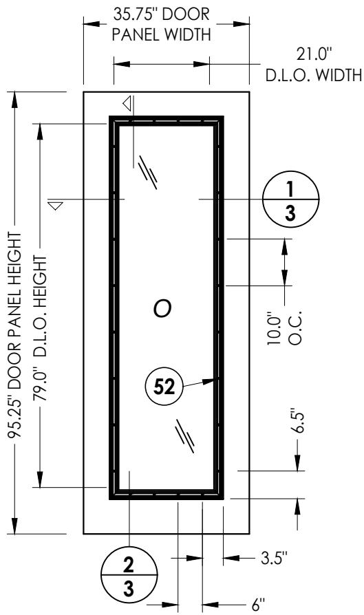
50 SIDELITE PANEL
