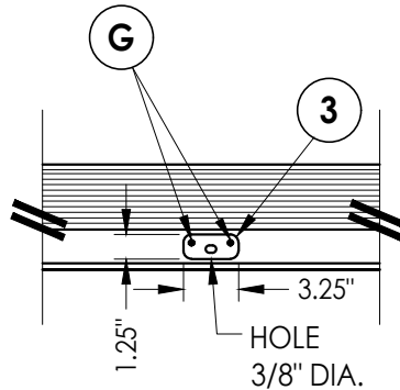
DETAIL 1 Inswing configuration
