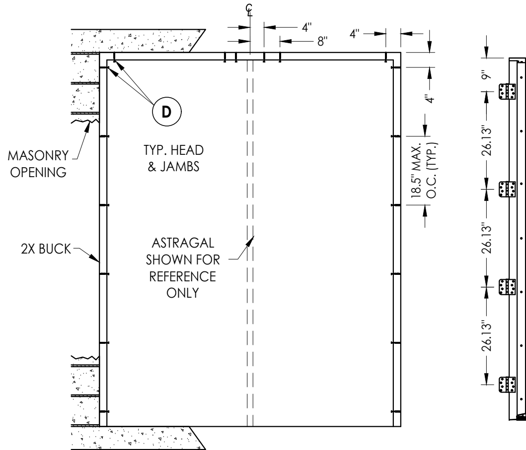
BUCK ANCHORING
